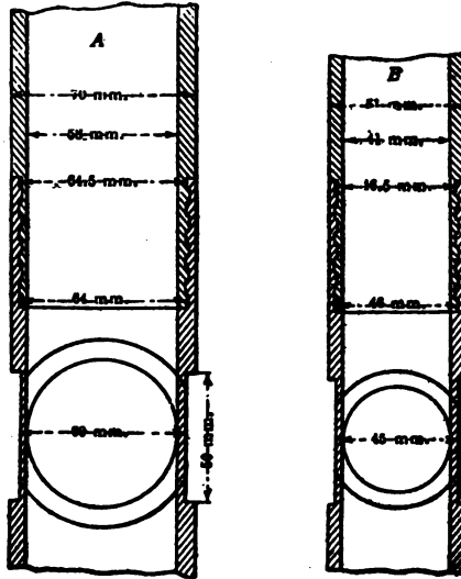
Fig. 72. Sections of Drill Rods.
